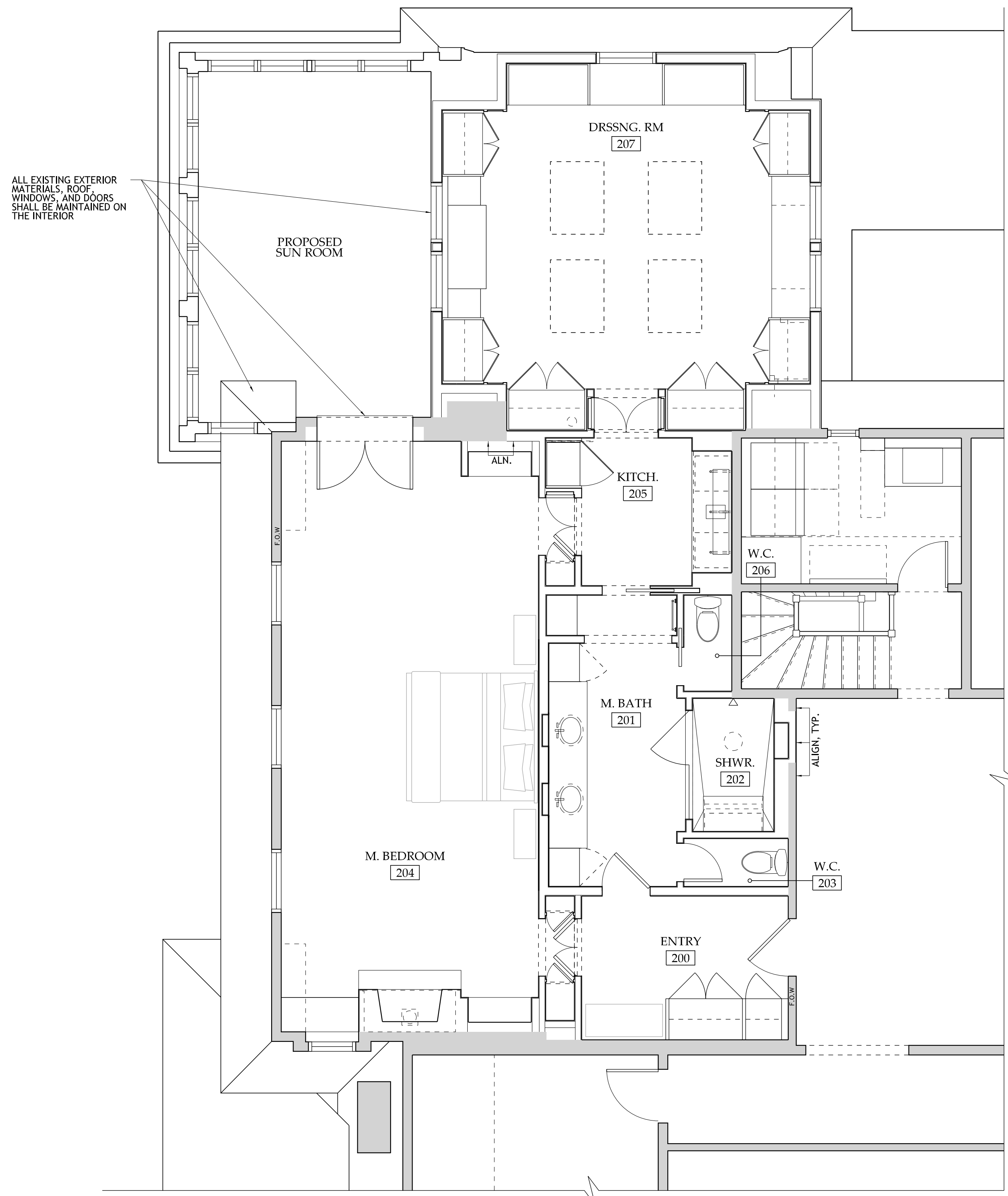
1 A101 PROPOSED SECOND FLOOR PLAN SCALE: 1/4" = 1'-0"
