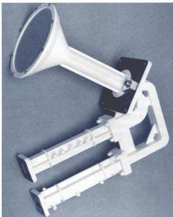
Figure 20. K_U -band feed system components are amenable to high-quantity/low-cost fabrication
