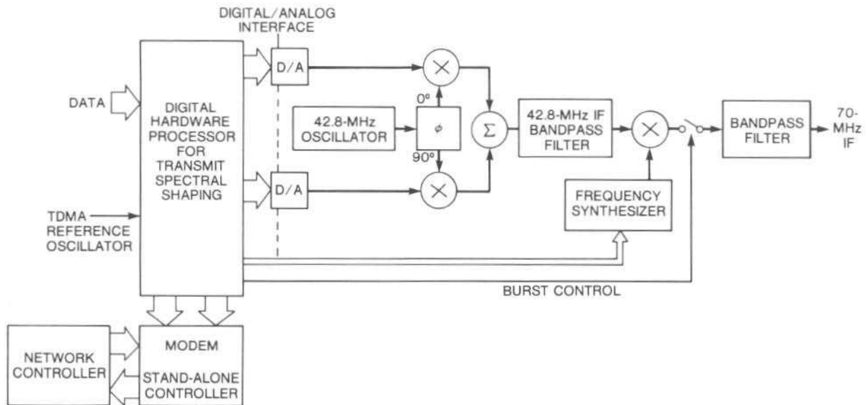
Figure 10. LR-TDMA modulator
