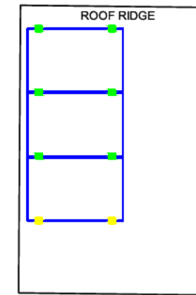
SOLAR PANEL FOOTING PLAN R3 Scale: 1/8" = 1'-0"
