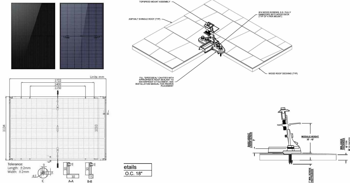
Figure 5: The specifications for the solar panels (left), and the installation details for the SnapNrack mounts (right).
