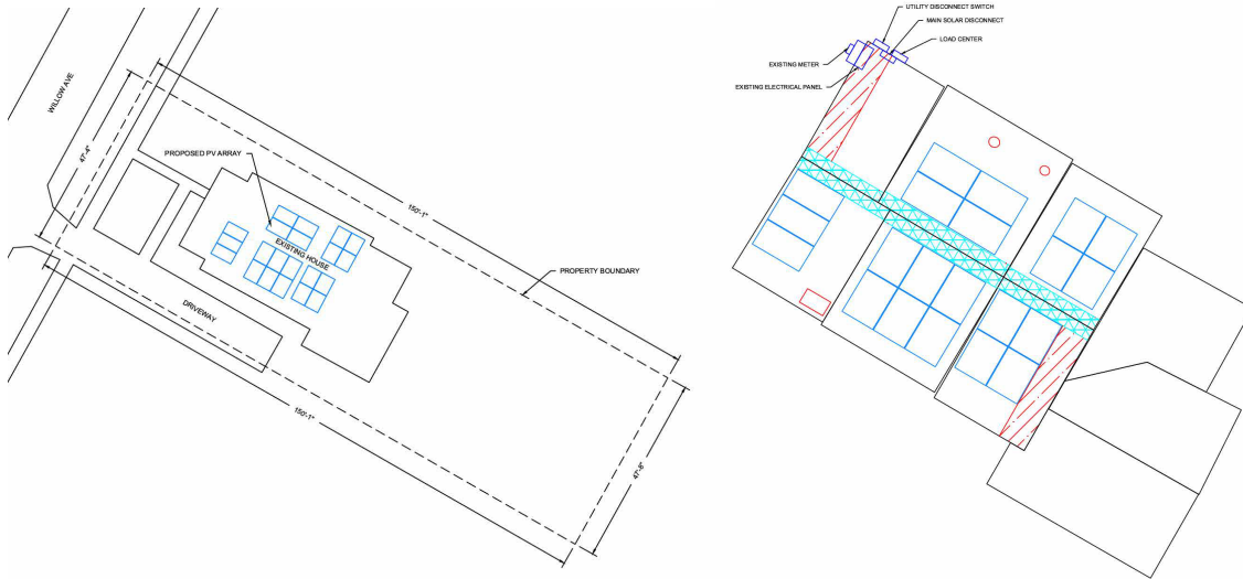
Figure 4: The site plan (left) shows the proposed solar panel locations and the building’s orientation toward Willow Avenue. The roof plan (right) shows the proposed location of the solar panels and the equipment location on the left-side elevation near the front wall plane.
