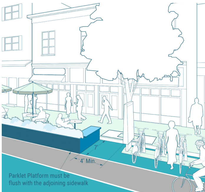
Figure 4-11. Illustration of parklet dimensions
