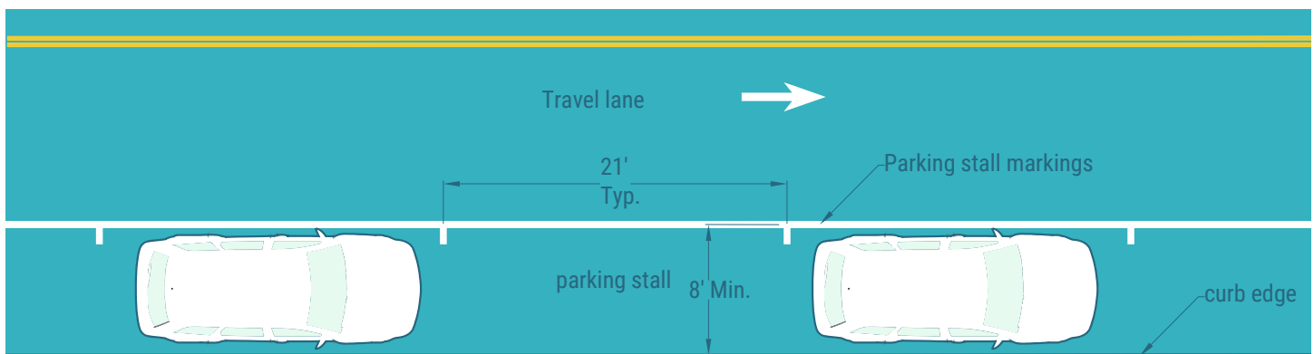
Figure 4-6. Illustration of a typical on-street parallel parking space with dimensions
