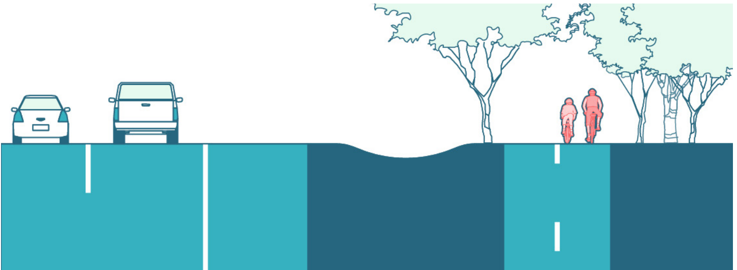
Figure 5-14. Sidepath Both Sides, 10' street buffer: Controlled Major Highway
