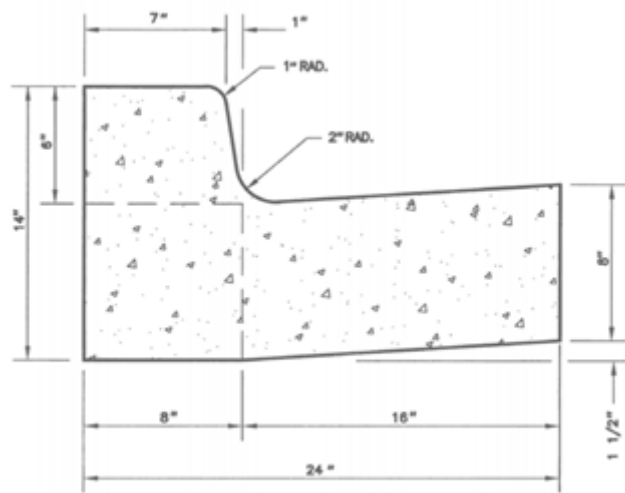
Figure 4-16. Montgomery County curb and gutter dimensions
