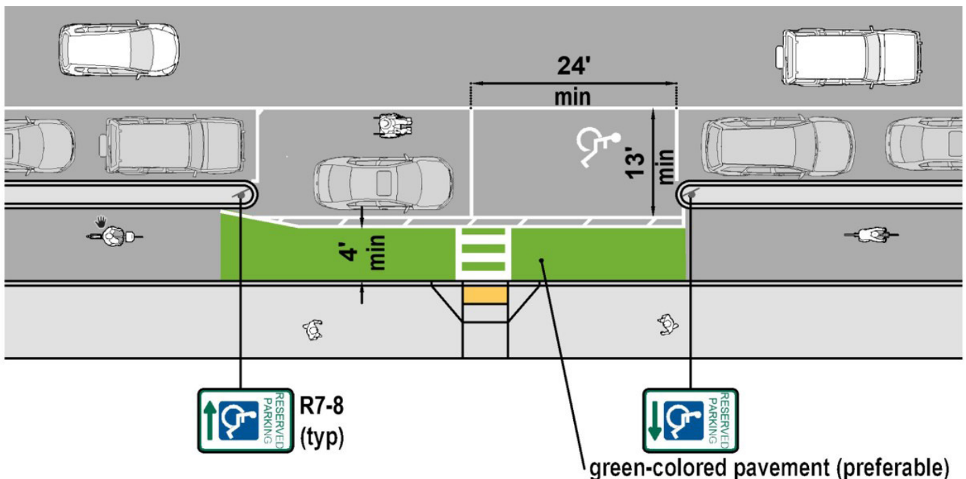
Figure 4-14. Example guidance for accessible passenger loading zone with a separated bike lane
