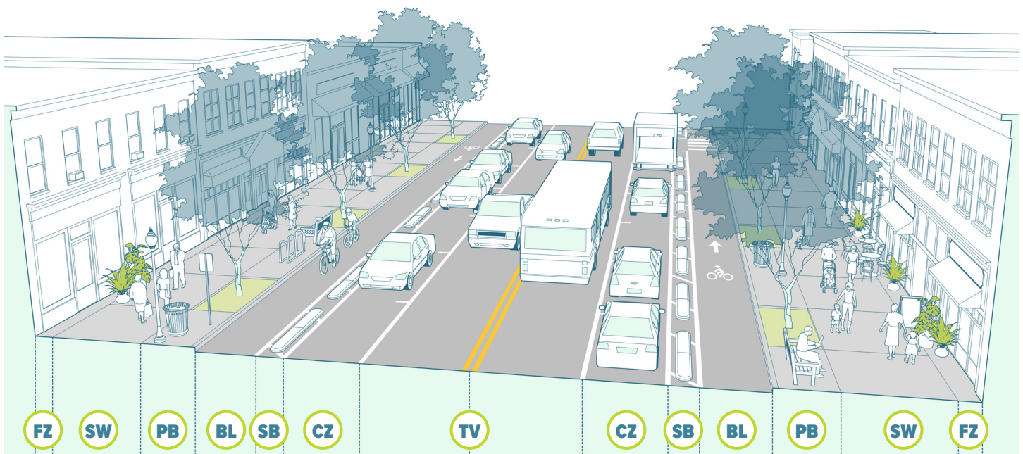
Figure 2-35. Town Center Street
