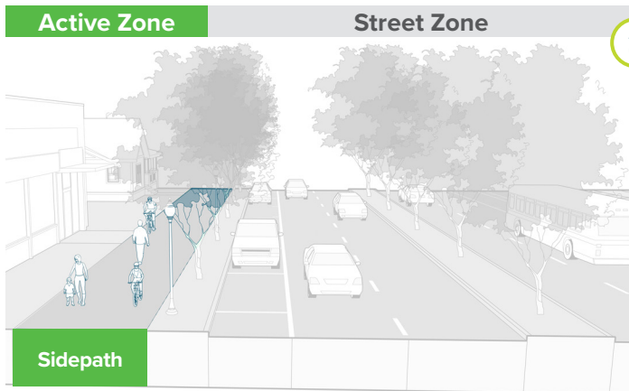
Figure 2-10. Sidepath
