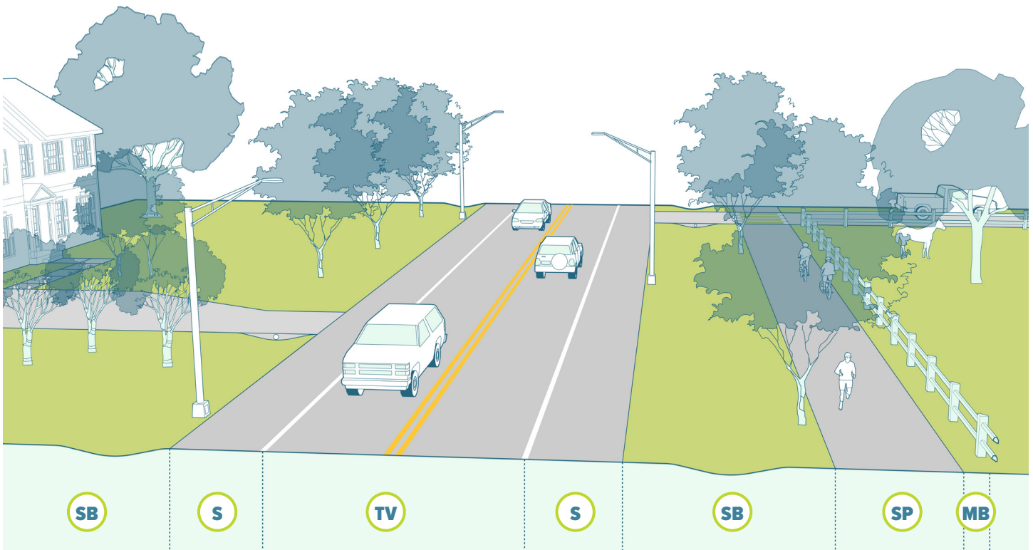
Figure 2-91. Country Road
