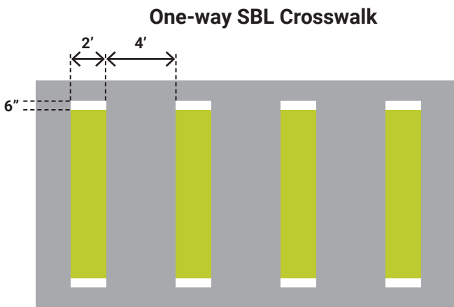
Figure 6-22. Bike crossing detail from Montgomery County Bicycle Master Plan
