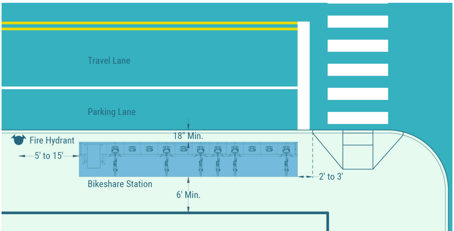
Figure 3-8. Example of bikeshare station clearance along and potentially within a Clear Zone (Graphic modified from NACTO Bike Share Station Siting Guide, https://nacto.org/publication/bike-share-station-siting-guide/ )
