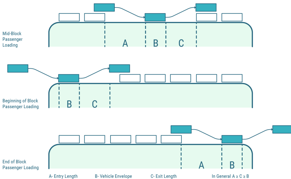
Figure 4-13. Ride hailing pickup/drop-off area diagrams (Graphic content from: ITE Curbside Management Practitioners Guide)
