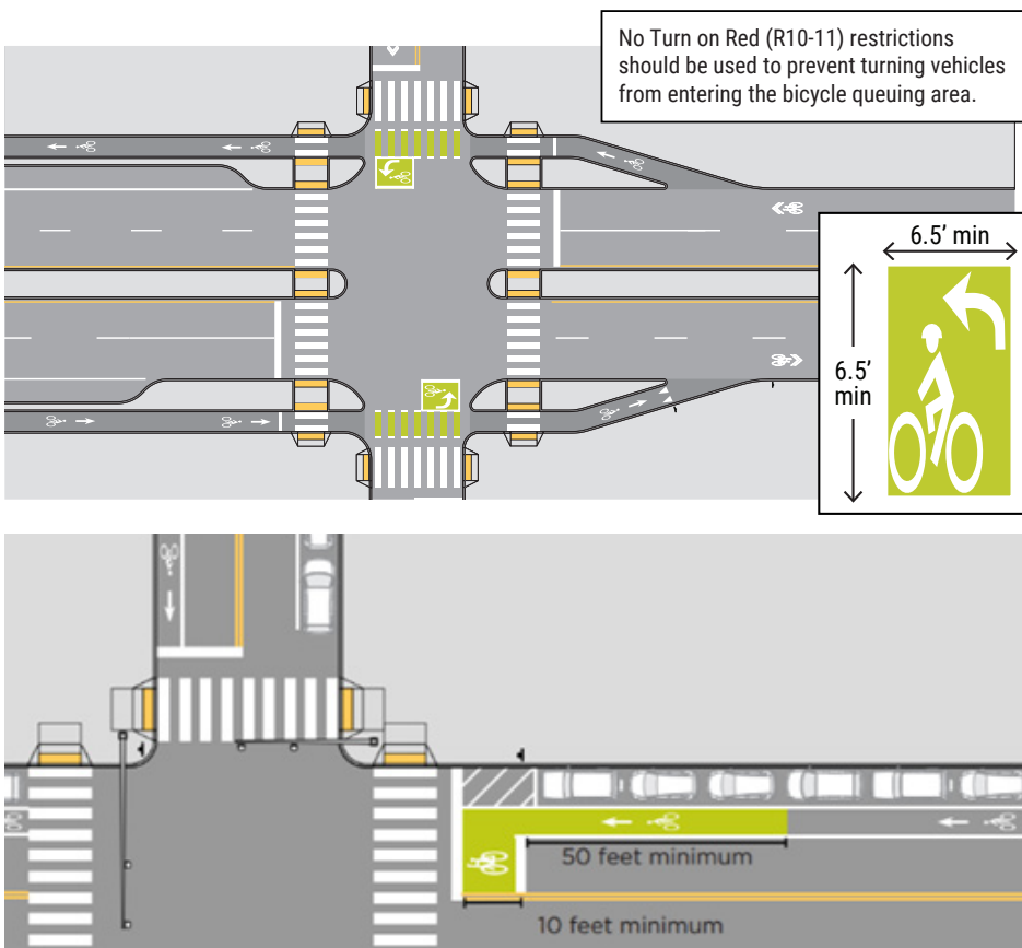
Figure 6-20. Two-stage turn queue box within a partially protected intersection example from Montgomery County Bicycle Master Plan Appendix B: Facility Toolkit
