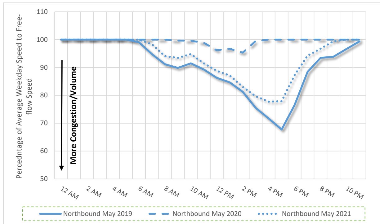
Figure 5: Average Weekday Speed as a Percentage of Free-Flow Speed (Northbound)
