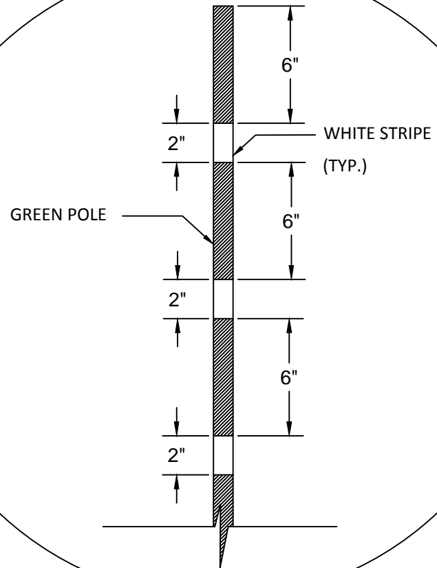
POLE STRIPING DETAIL
