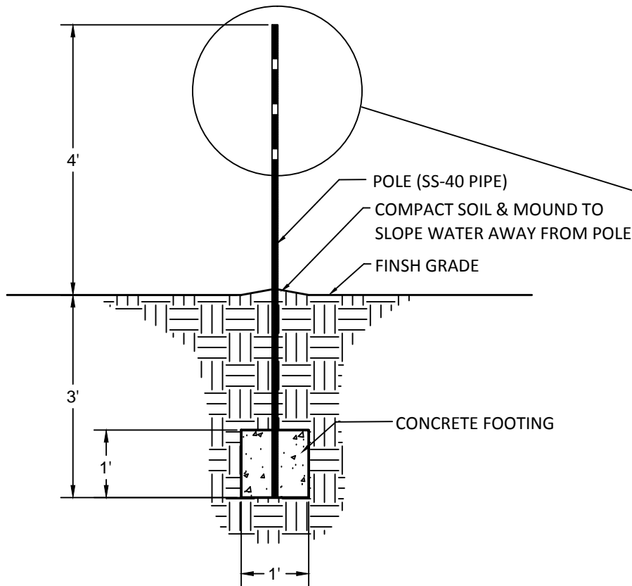
POLE INSTALLATION DETAIL
