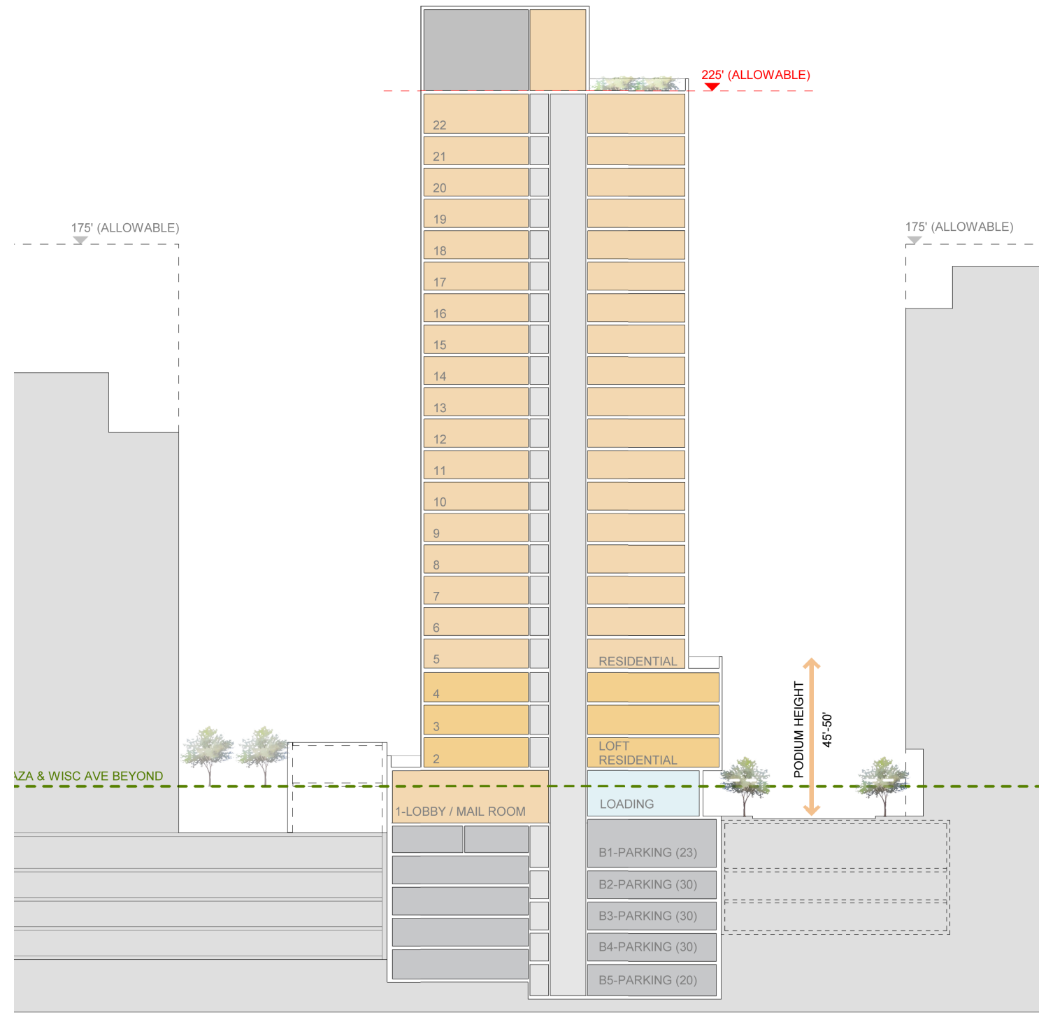
BUILDING SECTION
